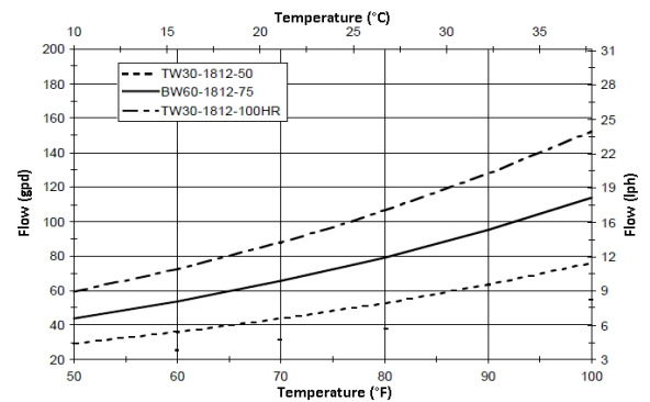
Figure 2: Impact of temperature on permeate flow (constant pressure, recovery)
